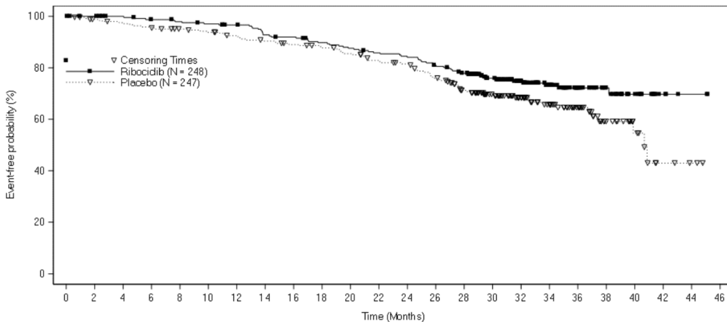
Figure 3 Kaplan-Meier Overall Survival Curves- MONALEESA-7 (NSAI)
